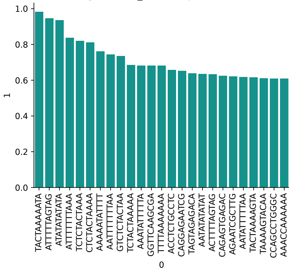
Isgkm K562_95033 Top 25 kmers
